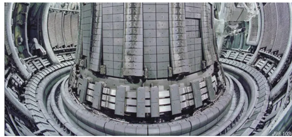
The toroidal magnetic chamber (Tokamak) of the Joint European Torus (JET) at the Culham Science Centre. Photograph: AFP/Getty Images
