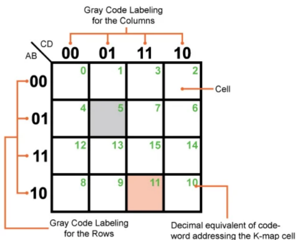
Figure 1: A typical but empty Karnaugh map with 16 cells
